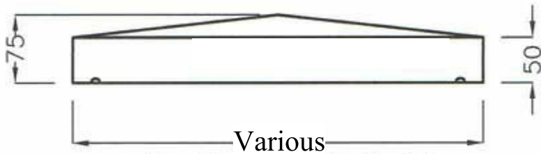
Elevation-Height Option P1/A
